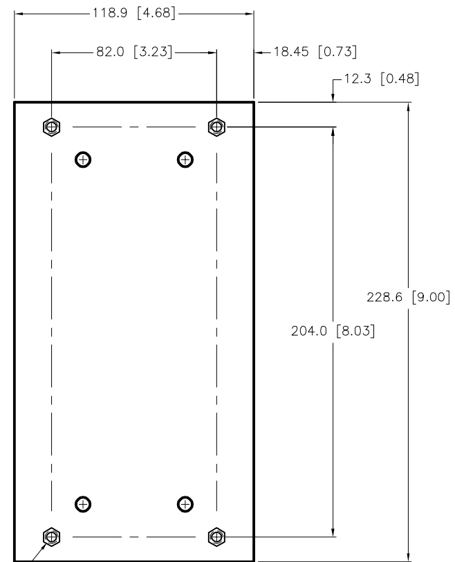
BOTTOM VIEW
